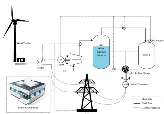
Figure 1. Schematic of the presented system connected to the wind farm and the grid
