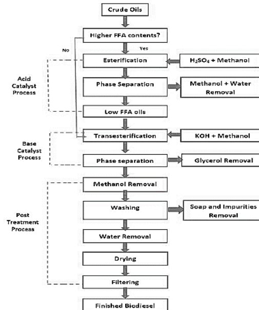
Figure 1. The flow chart of biodiesel production process [6].
